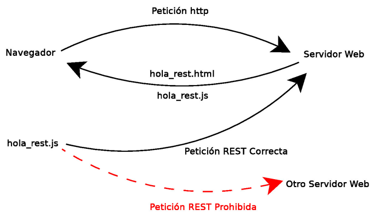
Figura 1: Same-Origin Policy
