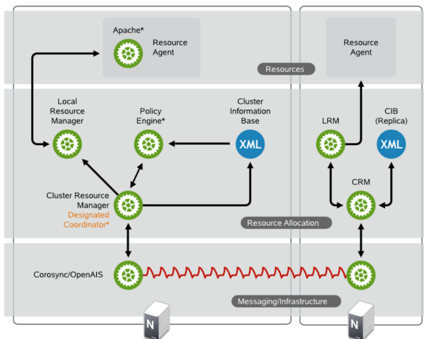
Figure 3.4: SUSE HA Cluster Components
