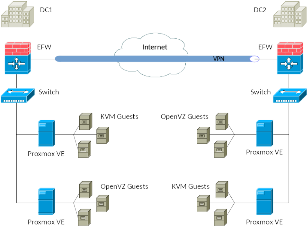
Figure 5.1: Network interconnection scheme
