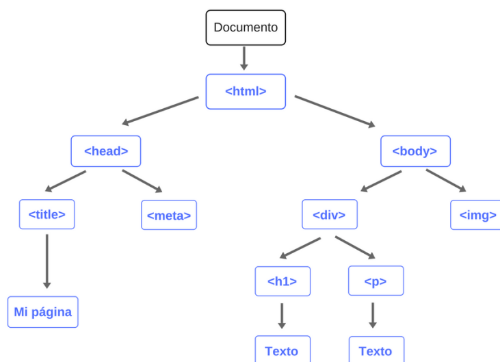
Figura 3.6: Document Object Model
