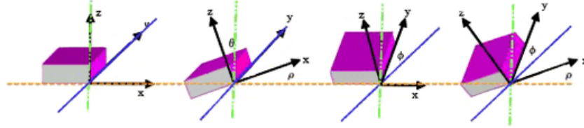
Figure 2.25: Trigonometry in accelerometer system 3D.
