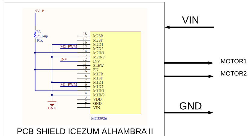
Figure 3.39: Schematic MC33926.
