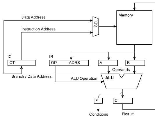
Figure 2.15: Basic architecture in a processor
