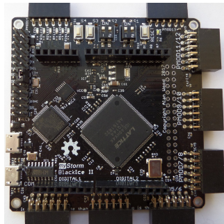
Figure 2.7: BlackIce II
