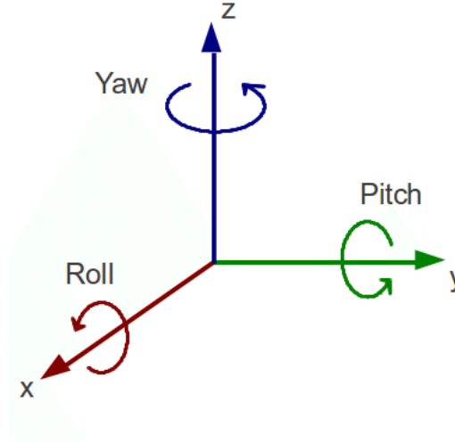
Figure 2.20: Tait-Brain angles.
