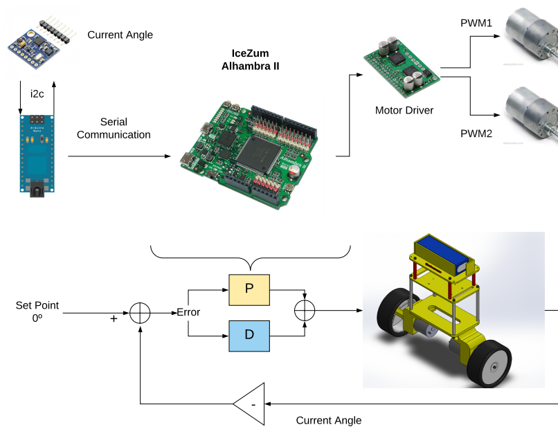
Figure 3.3: Final block diagram.
