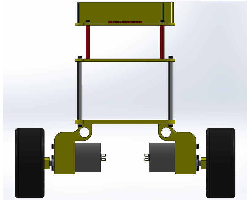
Figure 3.4: Frontal view Balancing Robot.
