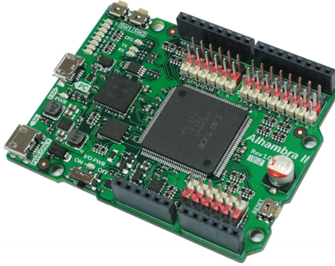
Figure 2.10: IceZUM Alhambra II Board
