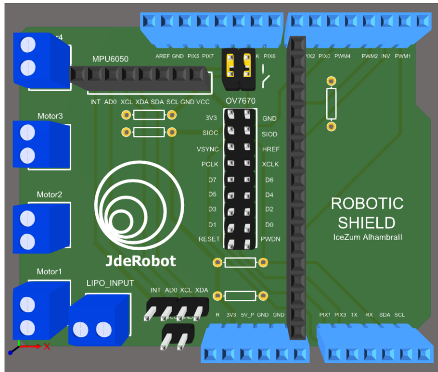
Figure 3.15: 3D View of Shield for IceZum Alhambra II.
