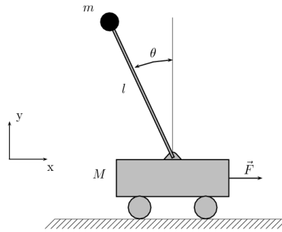
Figure 3.2: Inverted pendulum representation.
