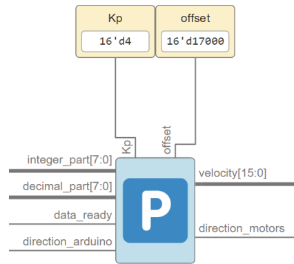
Figure 3.33: Appearance of P control in IceStudio
