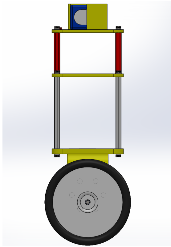
Figure 3.5: Lateral view derecha Balancing Robot.
