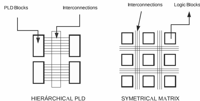
Figure 2.3: PLD vs FPGA
