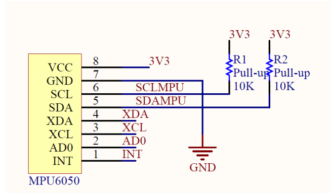
Figure 3.9: MPU6050 IMU.
