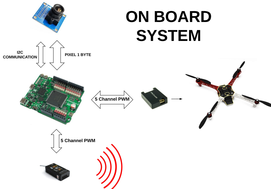
Figure 4.1: Vision quad-copter high level design.
