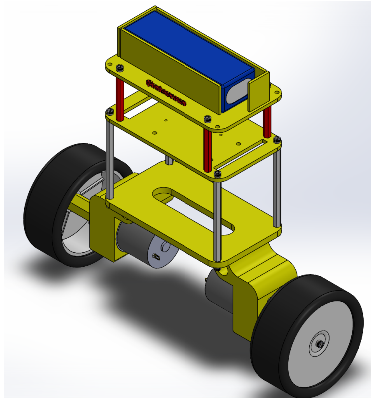
Figure 3.6: Balancing Robot perspective.
