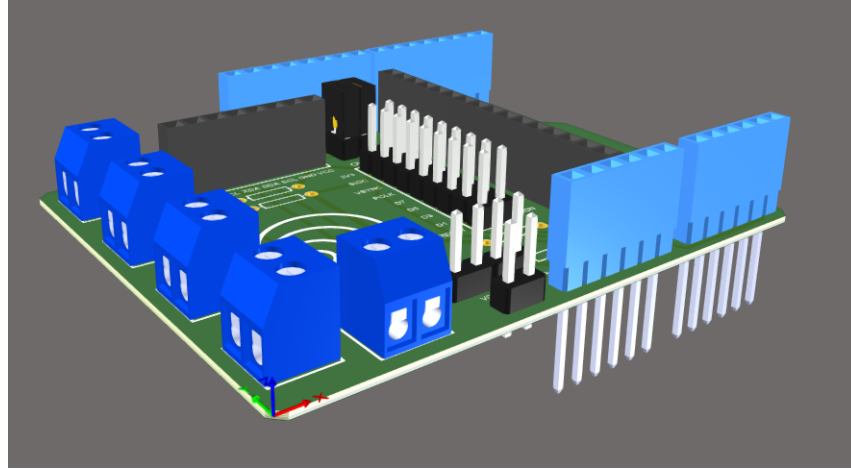
Figure 3.18: 3D of shield for IceZum Alhambra II.
