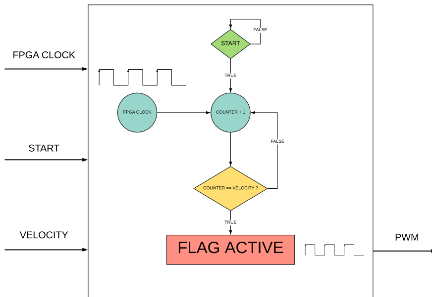
Figure 3.41: Flow diagram PWM generator in Verilog.
