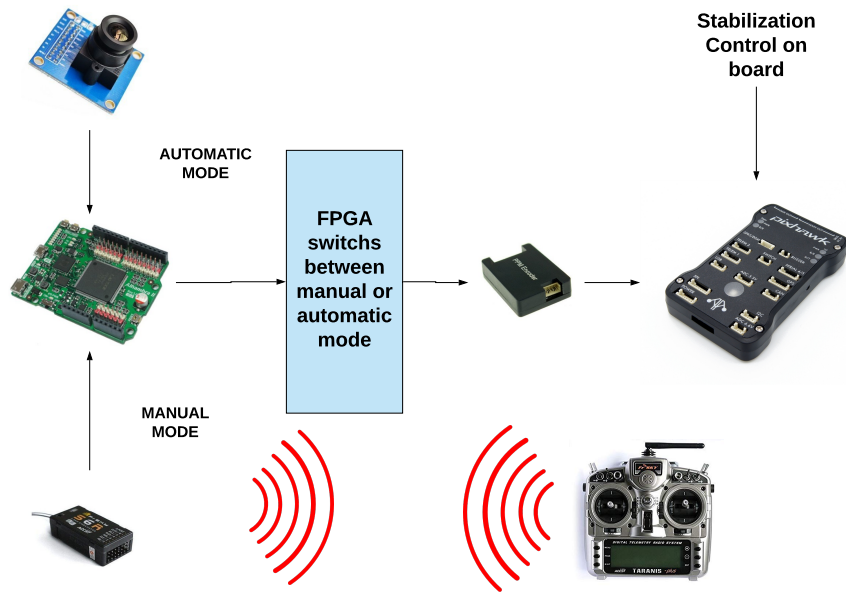
Figure 4.17: Diagram of control Implementation.
