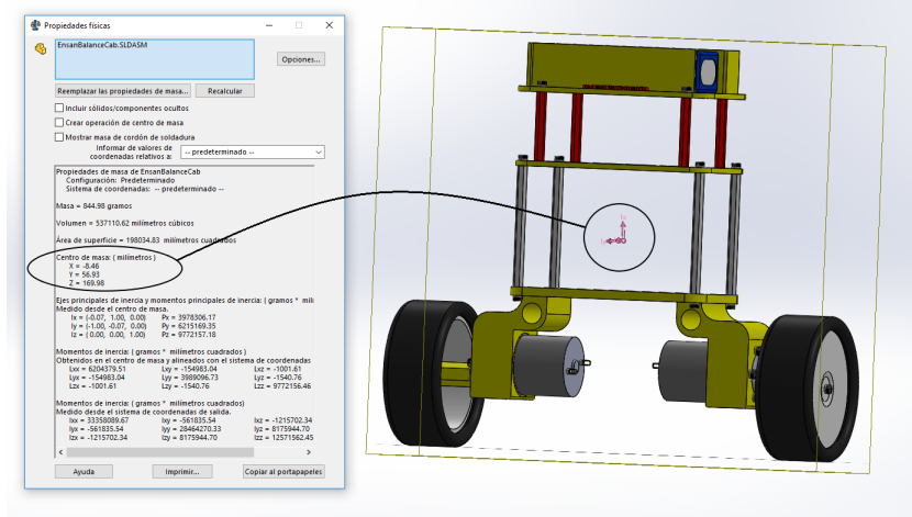
Figure 3.7: Center of mass final system.
