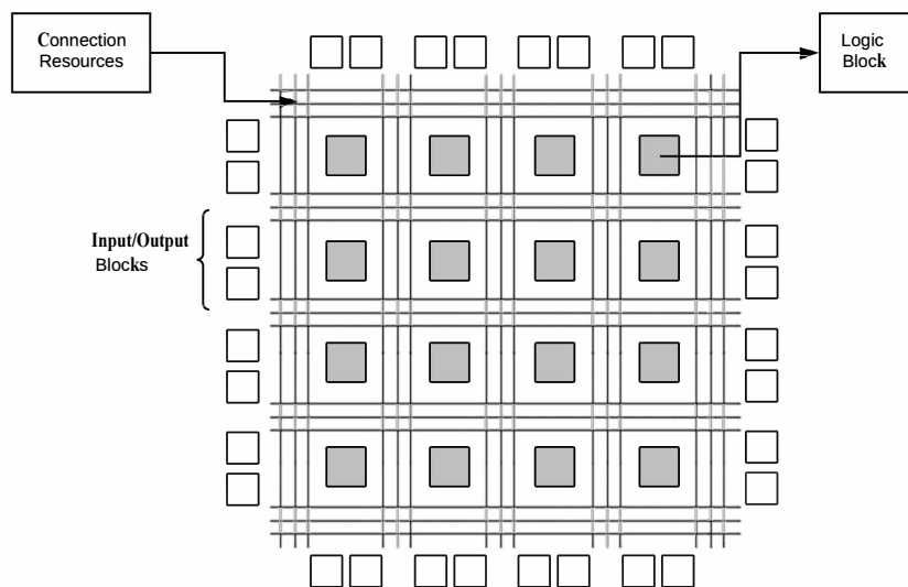
Figure 2.1: PLD vs FPGA
