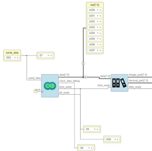
Figure 3.31: Communication between Arduino and IceZum Alhambra.
