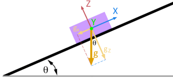
Figure 2.24: Trigonometry in accelerometer system 2D.
