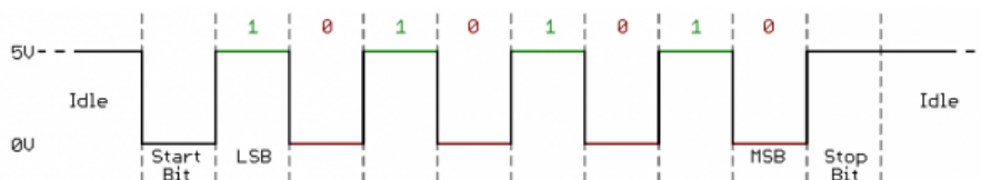
Figure 3.22: Serial communication example.
