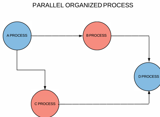
Figure 2.4: Process Parallelism
