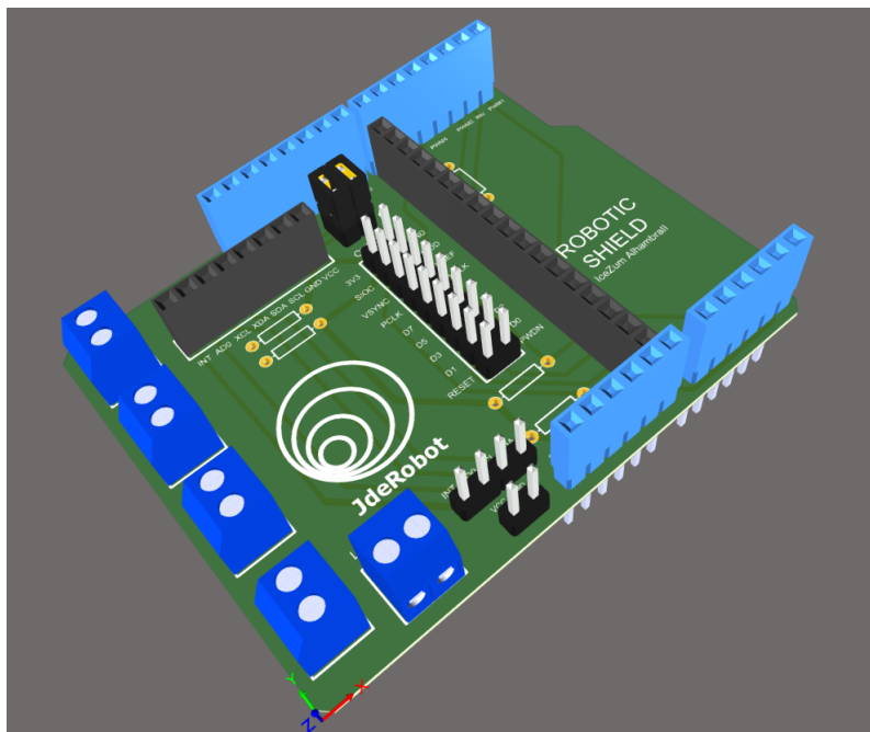
Figure 3.17: 3D of shield for IceZum Alhambra II.
