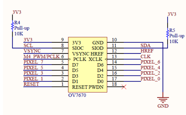
Figure 4.6: OV7670 camera schematics.
