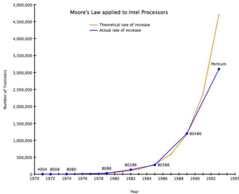
Figure 2.2: Moore's Law
