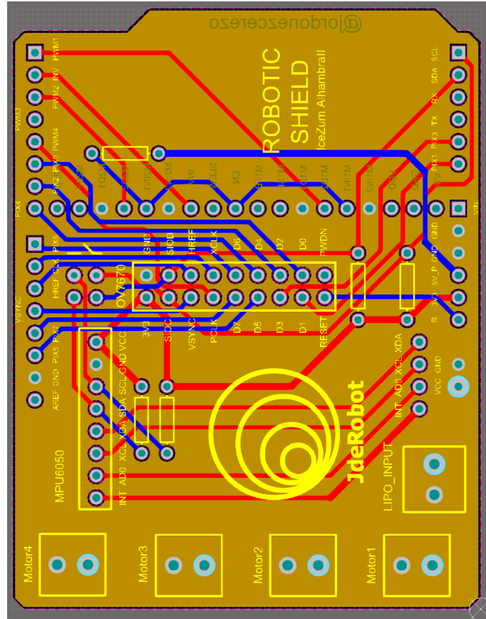
Figure 3.20: Composition layers in Altium.
