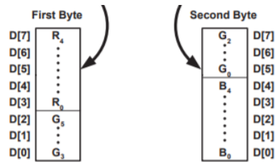
Figure 4.3: OV7670 Pixel Formation
