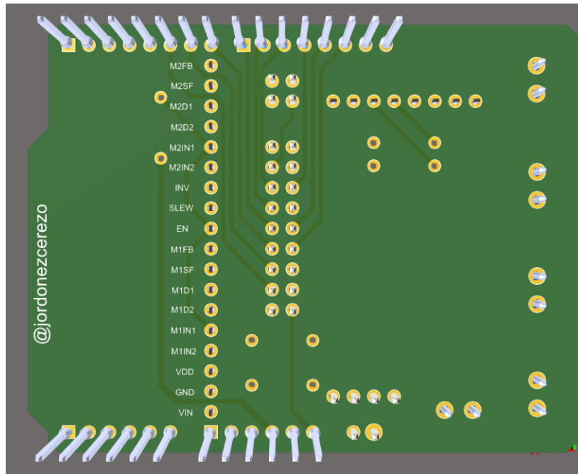
Figure 3.16: 3D View of Shield for IceZum Alhambra II.
