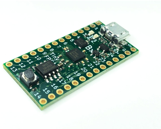
Figure 2.6: Tiny FPGA BX
