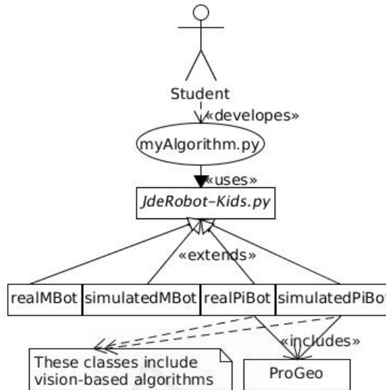
Figure 4.8: The student uses the JdeRobot-Kids.py library in his program
