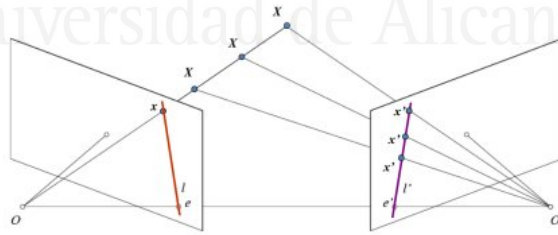
Figure 4.11: Cameras taking an image from the same scene
