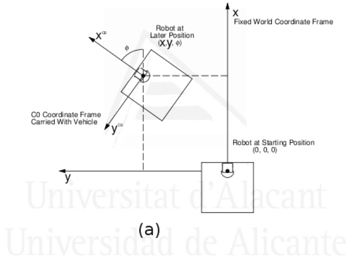
Figure 3.5: C0 coordinate system
