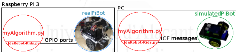
Figure 4.10: Connection of the JdeRobot-Kids.py library with the real PiBot and with the simulated PiBot
