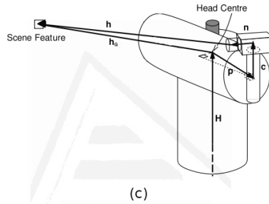
Figure 3.7: C3 coordinate system
