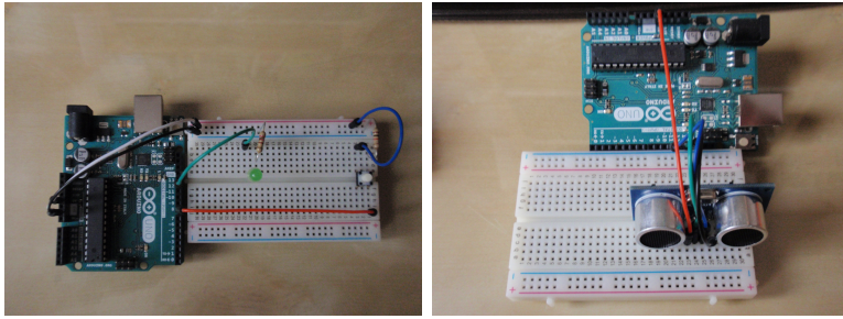
Figure 4.16: Practice task with Arduino to operate a push button with LED and ultrasonic
