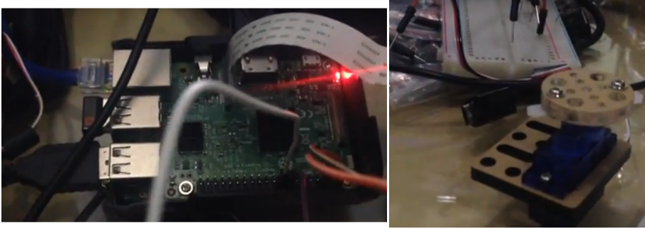
Figure 4.20: Practice task with PiBot to operate a servo
