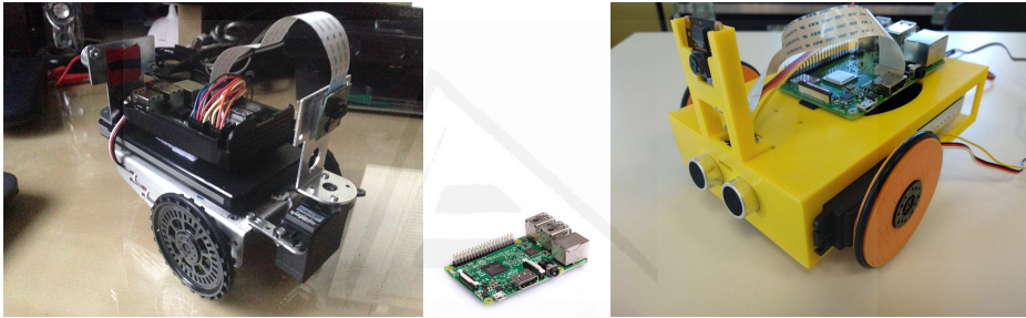
Figure 4.3: Robotic platforms PiBot (left) and PiBot made with 3D printable pieces (right), both of them based on Raspberry Pi 3 (middle)
