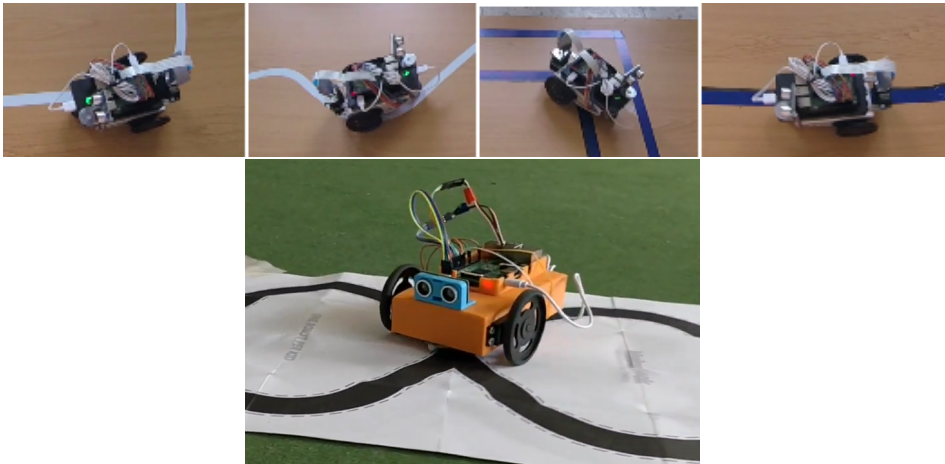
Figure 4.25: Practice line tracking task in different PiBot robots using infrared
