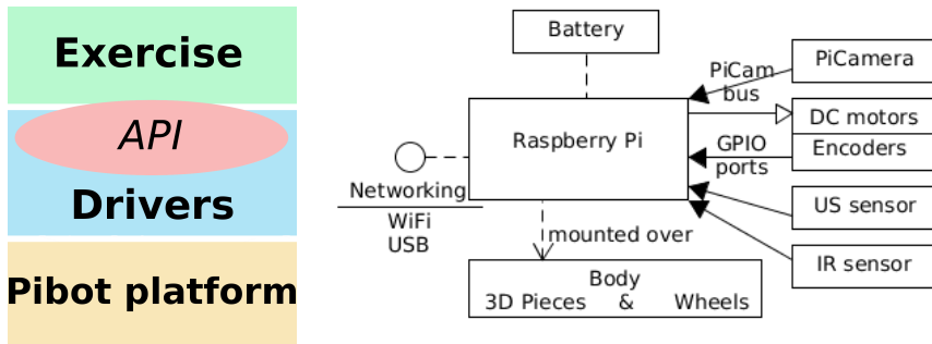
Figure 4.5: Architecture (left) and hardware design (right) of the PiBot
