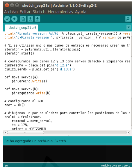
Figure 2.9: Program in Arduino IDE environment
