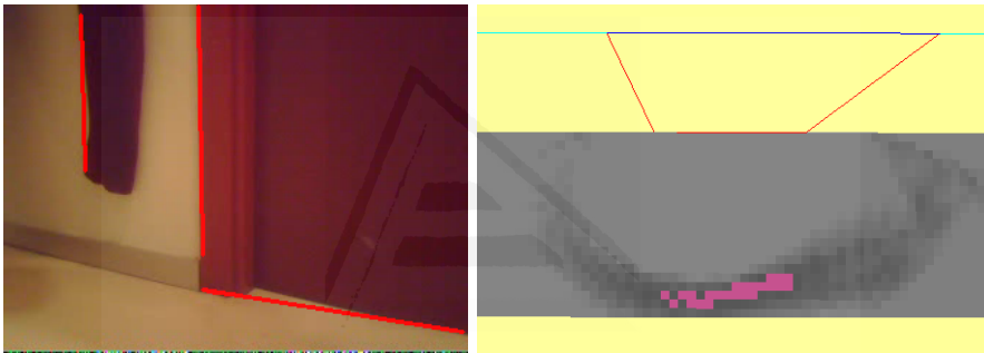
Figure 3.33: Observed image (left) and calculated probabilities with false positives for any \theta (right)
