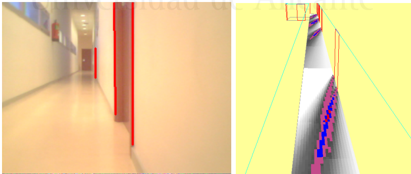
Figure 3.29: Observed image (left) and probabilities calculated with \theta equals to 0 radians(right)
