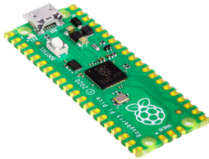
(a) Raspberry Pi Pico
